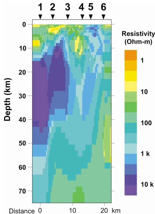
Fig. 6. Geoelectric cross section over the Middle Andaman region.
