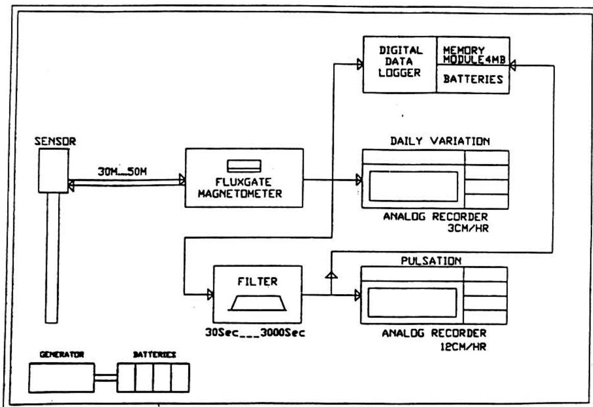
Fig.2: Block diagram of the fluxgate magnetometer set-up used at the three locations. The data is acquired in both analog and digital form
