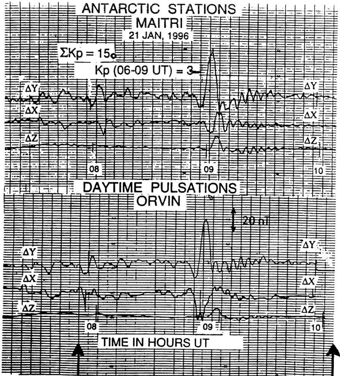
Fig.3a: Simultaneous geomagnetic pulsations experienced at the two locations MAI and OR on 21 Jan 1996 between 0800 and 1000 UT. The drift speeds of the small-scale ionospheric current systems are estimated from the time lags in similar pulsations
