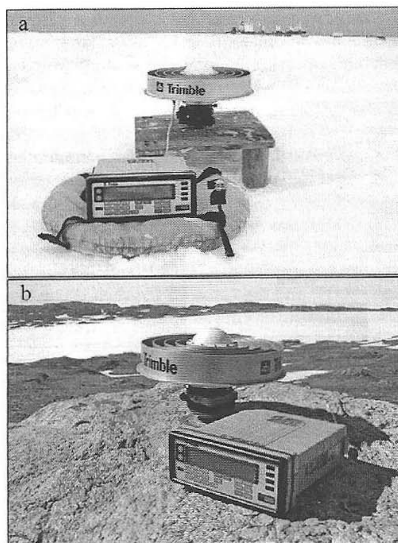
Fig. 2. (a) GPS antenna mounted on wooden platform on the glacier. (b) Set-up of the GPS base station on bedrock.
