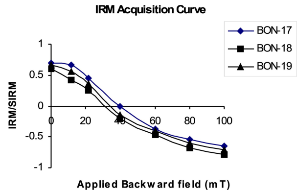
Fig. 3. Isothermal remanent magnetisation acquisition (back-field DC demagnetization curves).
